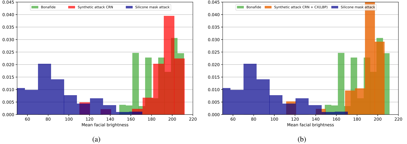
Figure 5: Score distribution of mean facial intensity baseline for bonafide and attack samples. (a) synthetic attack CRN (b) synthetic attack CRN+CX(LBP)
