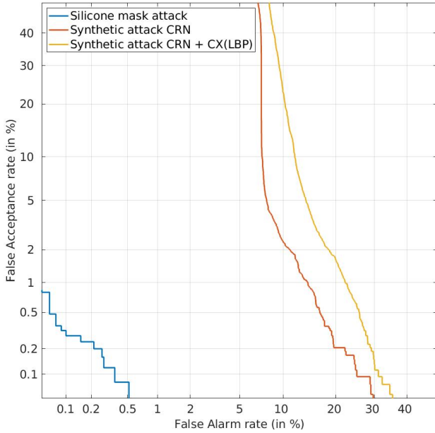
Figure 6: Detection error tradeoff (DET) curves of LBP+LR spoofing attack detection baseline for different attacks.
