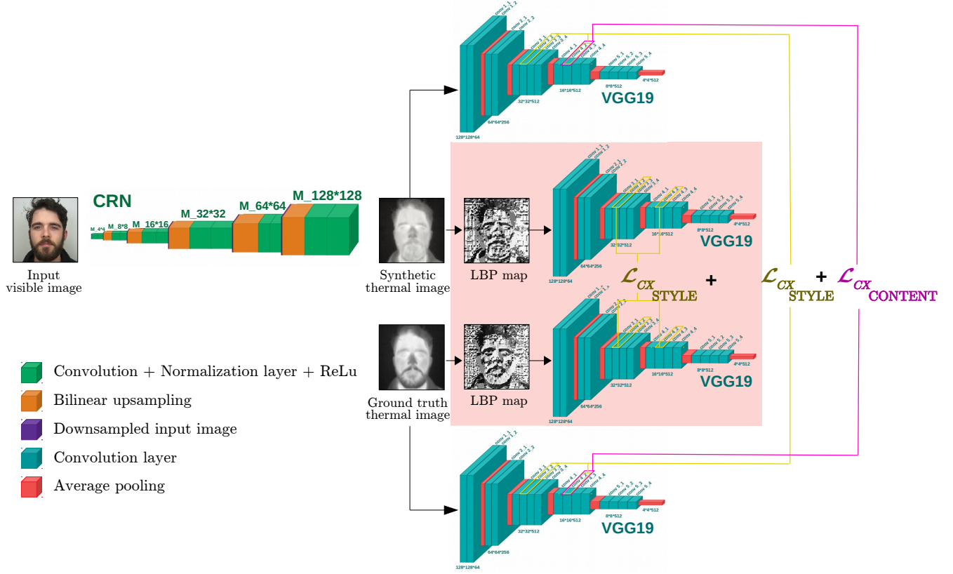
Figure 2: Illustration of the proposed architecture to perform visible-to-thermal spectrum conversion. The highlighted blocks of the diagram illustrate the introduced loss for the customised approach.
